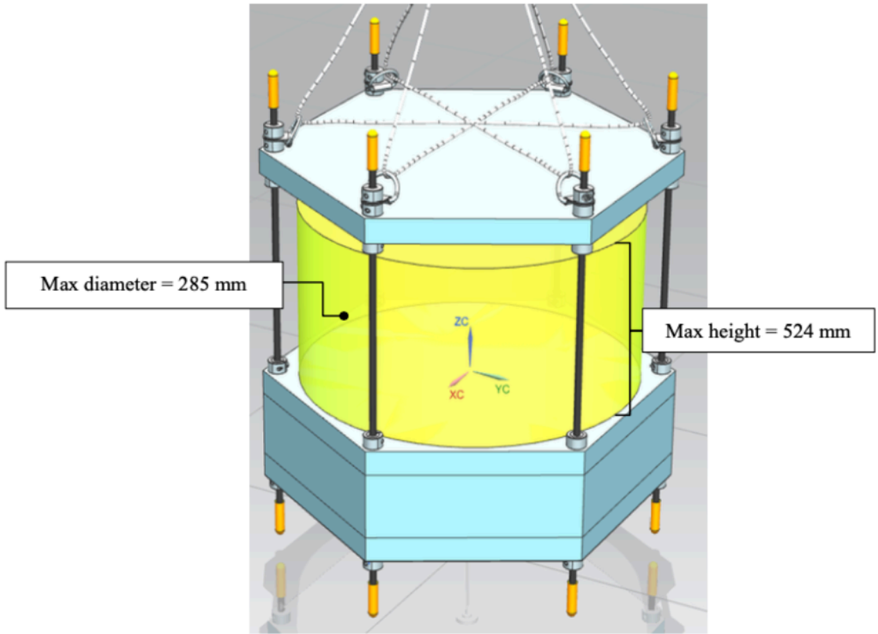
Figure 2.2: Payload volume constraint in yellow. Note that the payload must be clear of the 6 rods on the perimeter.
